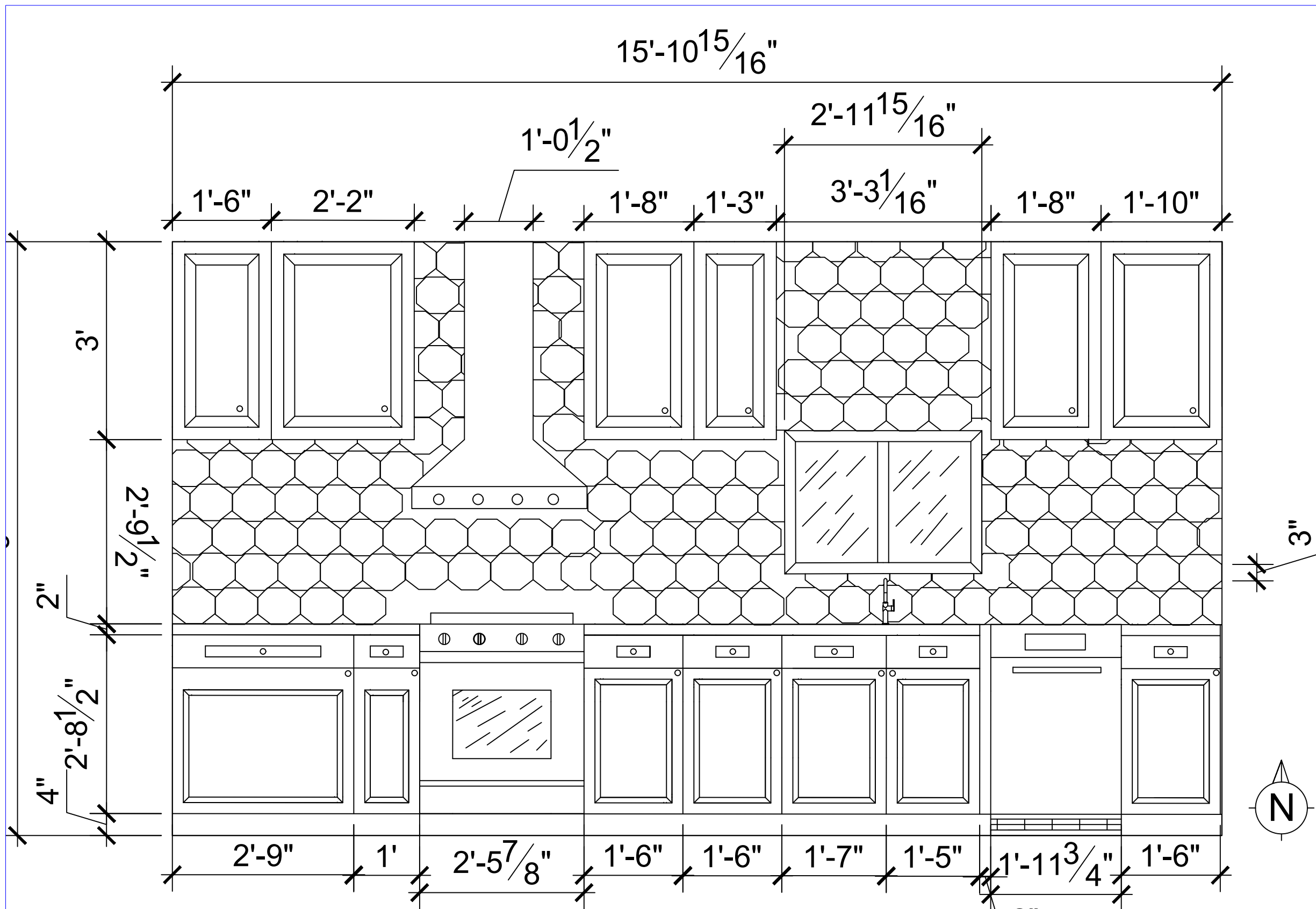
A ELEVATIONS
