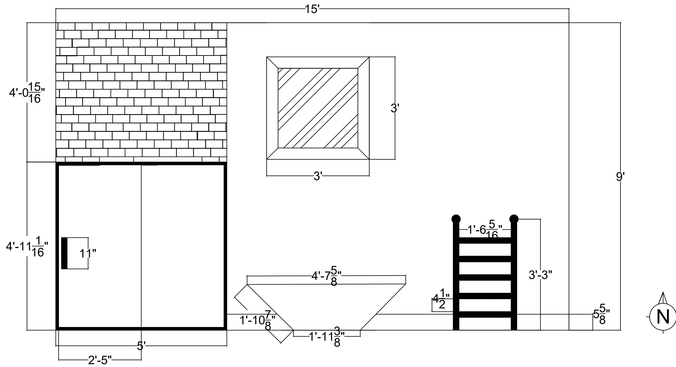
A ELEVATIONS
